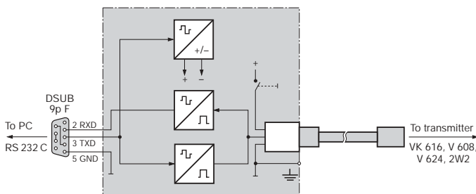
Fig. 2. Schematic diagram of the programming cable PK 610.
