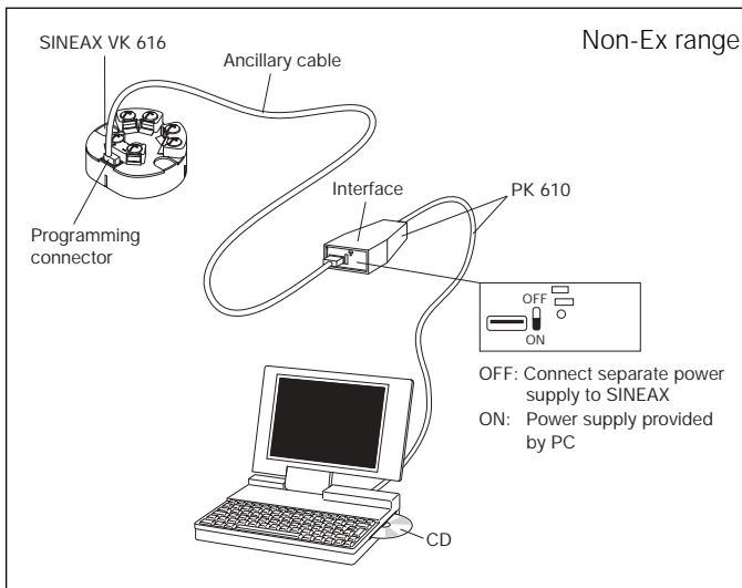
Fig. 1. Example for a connection for programming with a SINEAX VK 616 in standard version.
