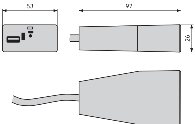
Fig. 7. Interface on the programming cable PK 610.
